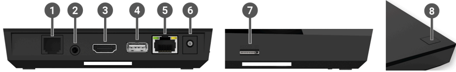
Figure 1: Connections
